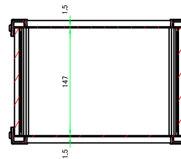
C-C (1:5)
